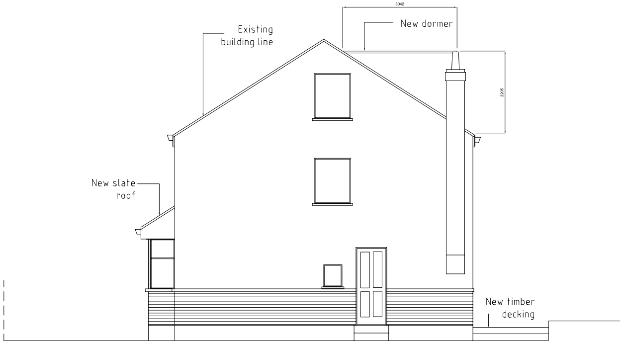
Proposed Side Elevation (Right)
