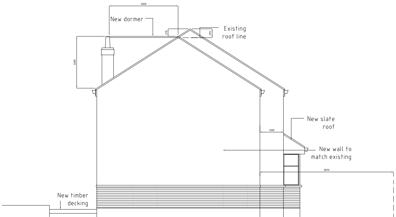
Proposed Side Elevation (Left)
